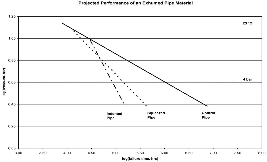
Figure 1: Project Performance of an Exhumed-from-Service PE Piping Material
